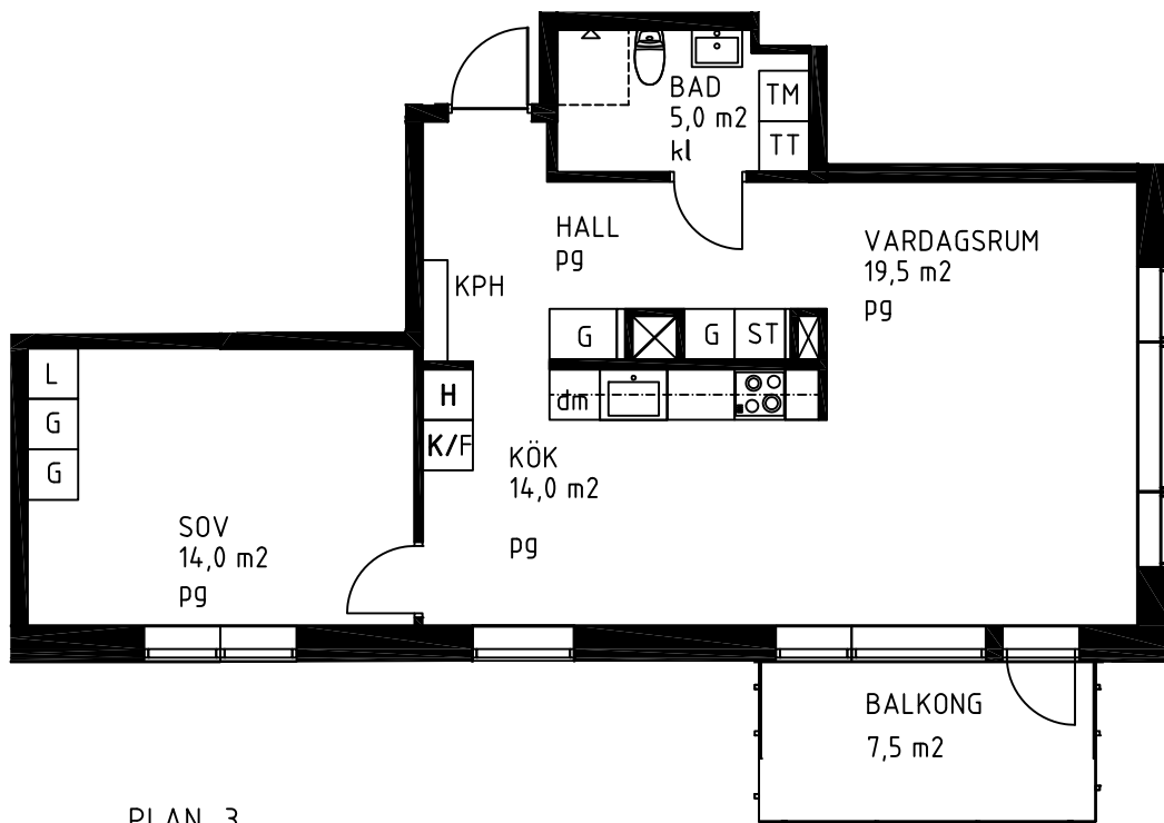
PLAN 3
