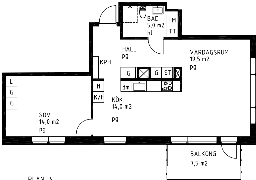
PLAN 4
