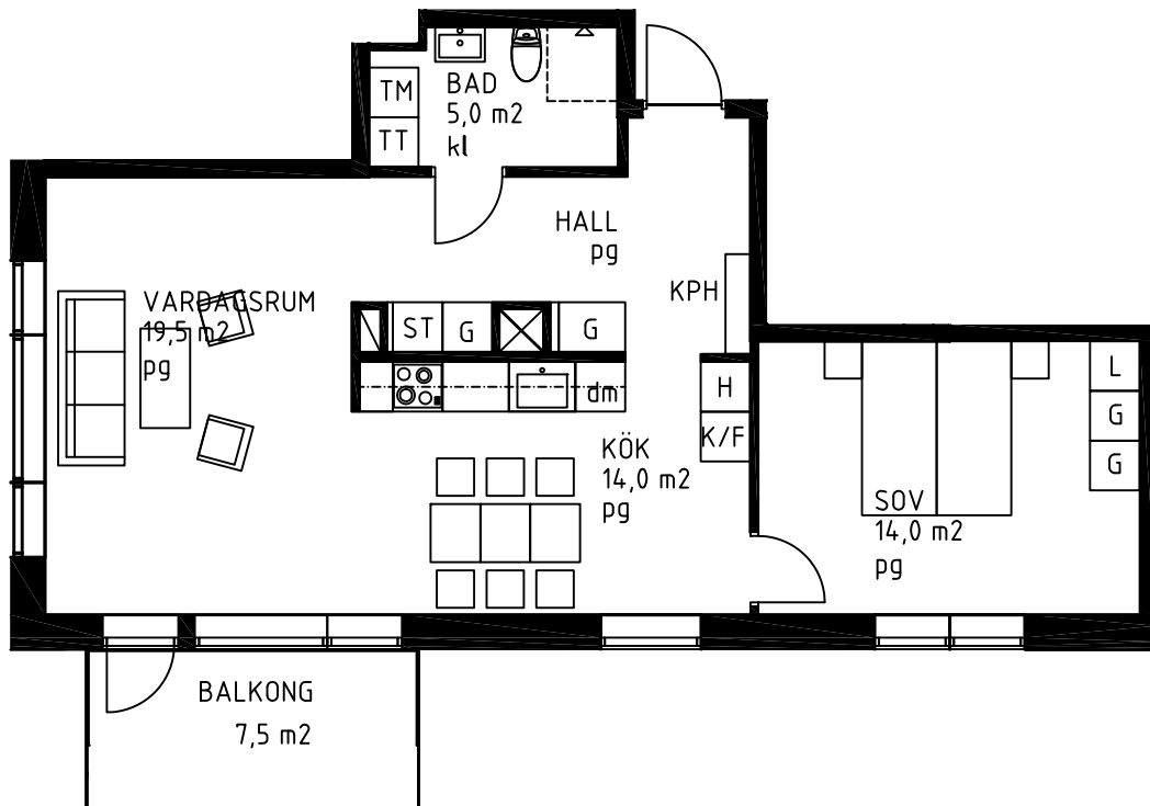
PLAN 3
